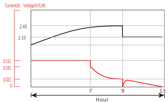
Charge performance
