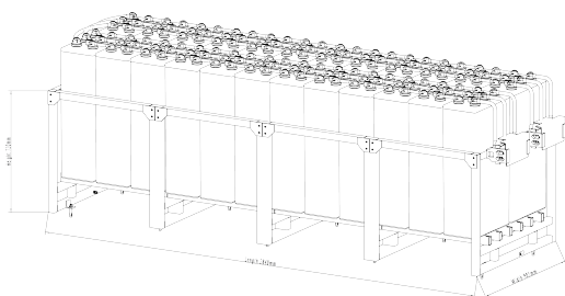
48V Standard Rack Rack material: powder-coated steel Height*width: 1*2 Ref. 16 OPzV 2000 Rack (approx. weight: 3900kg)
