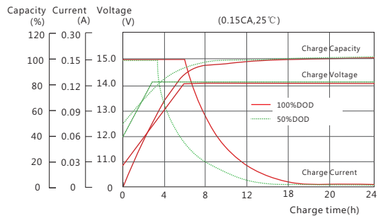
Charge performance
