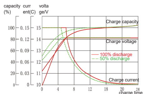
Charge performance
