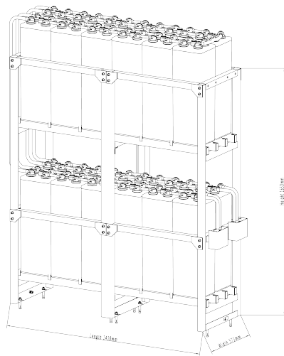
48V Standard Rack Rack material: powder-coated steel Height*width: 2*2 Ref. 10 OPzV 1000 Rack (approx. weight: 2020kg)
