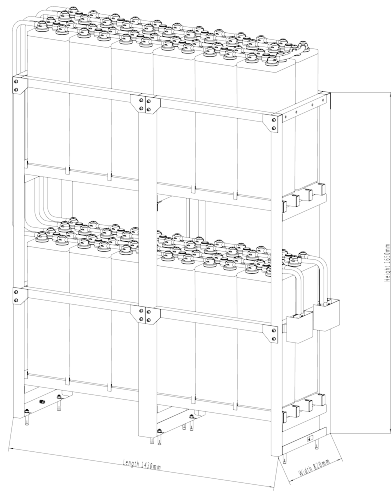
48V Standard Rack Rack material: powder-coated steel Height*width: 2*2 Ref. 15 OPzV 1500 Rack (approx. weight: 2900kg)
