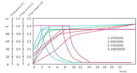
Charge vs. discharge depth
