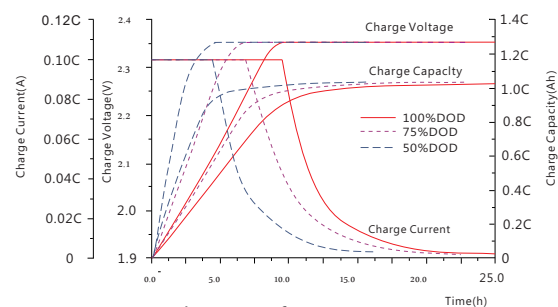
Charge performance
