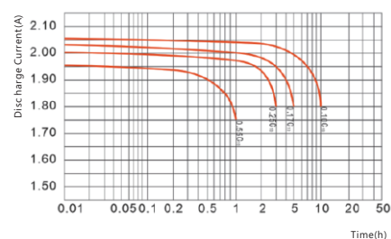
Discharge performance
