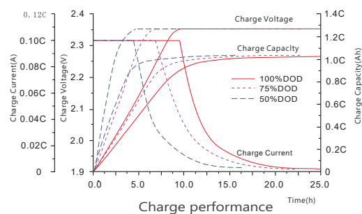
Charge performance
